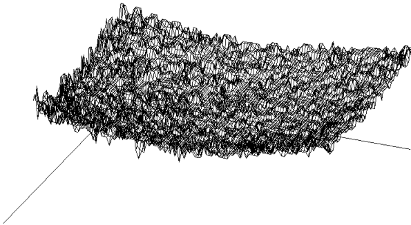
Figure 6: Depth image
