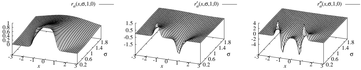
Figure 1: Scale-space behavior of the bar-shaped line f_a with a = 0 and w = 1 when convolved with the derivatives of Gaussian kernels for x \in [-3, 3] and \sigma \in [0.2, 2] .
