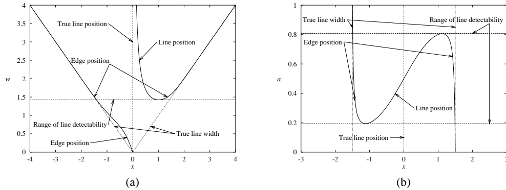
Figure 7: (a) Location of a staircase line with a = 0.75 , w \in [0, 4] and its edges for \sigma = 1 . (b) Location of a staircase line with w = 1.5 , a \in [0, 1] and its edges for \sigma = 1 .
