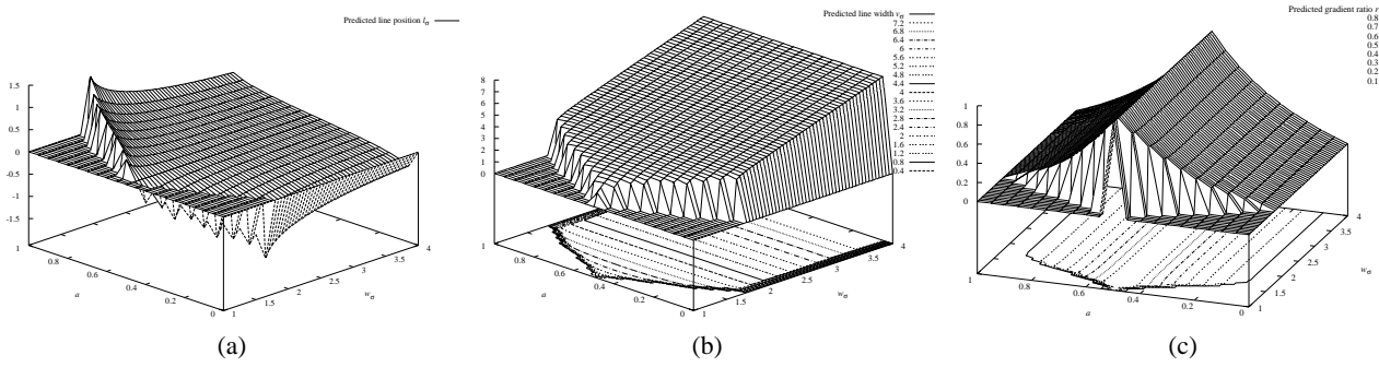
Figure 8: (a) Predicted line position l_\sigma of the staircase line f_s for w_\sigma \in [1, 4] and a \in [0, 1] . (b) Predicted line width. (c) Predicted gradient ratio r .
