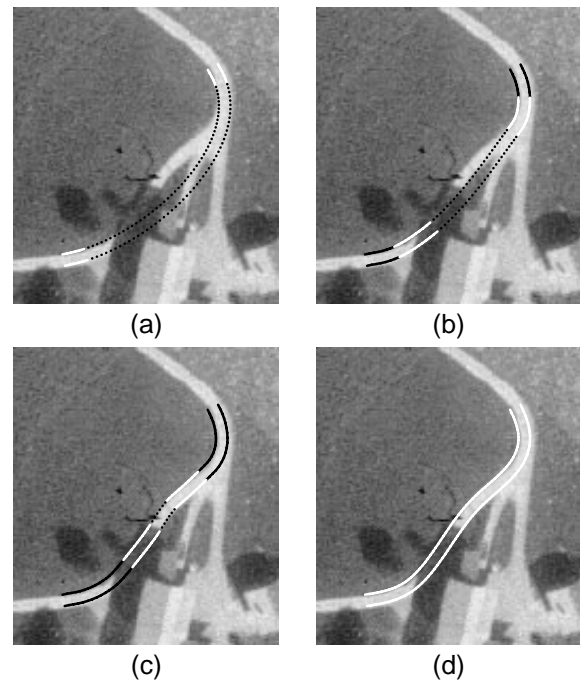
Figure 9: Optimization steps of a “zip-lock” ribbon. (a)-(c) Dotted lines indicate the passive part of the ribbon. White parts are currently optimized. Black ends indicate the result of the optimization so far. (d) Final result
