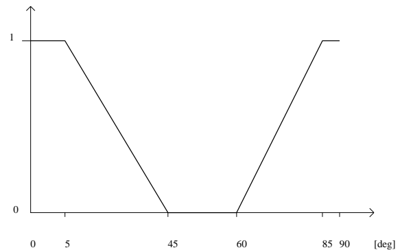
Figure 16: Fuzzy function for evaluating direction difference
